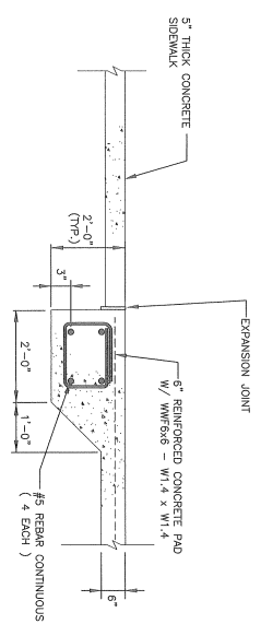
SHELTER PAD DETAIL NOT TO SCALE
