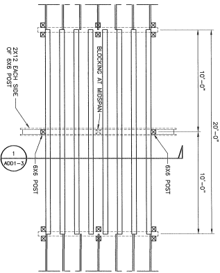
PARTIAL PLAN AT LONG SPAN OF BOARDWALK SCALE 1/4"=1'-0" SEE ORIGINAL SECTION FOR INFORMATION NOT SHOWN.
